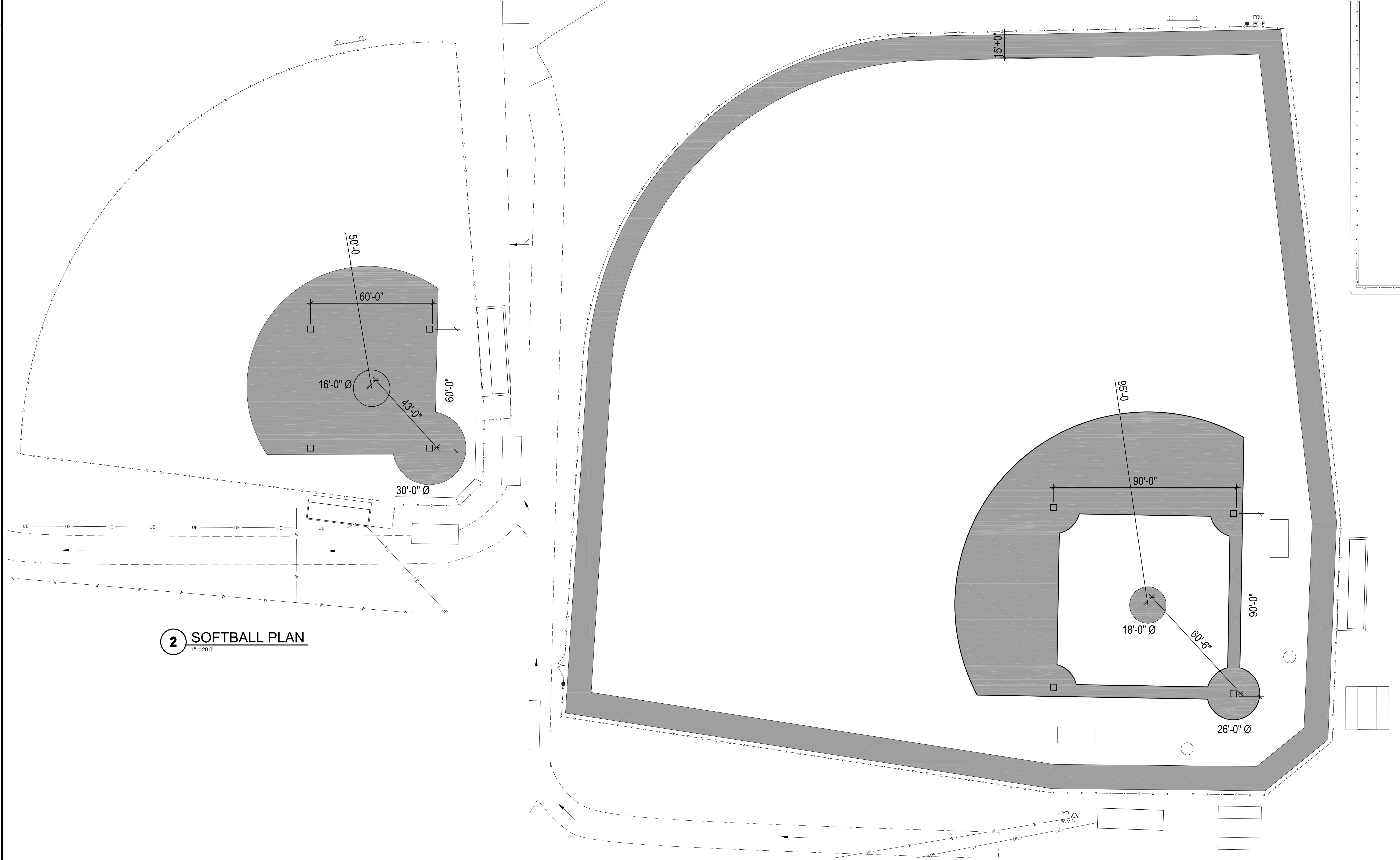
1 VARSITY BASEBALL PLAN 1" = 20.0'
